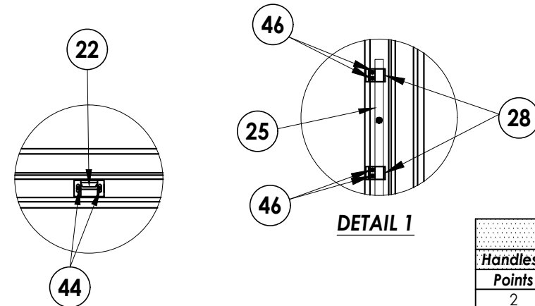
SNUBBER DETAIL
