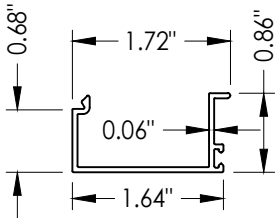
9 GLASS STOP 1/4"
