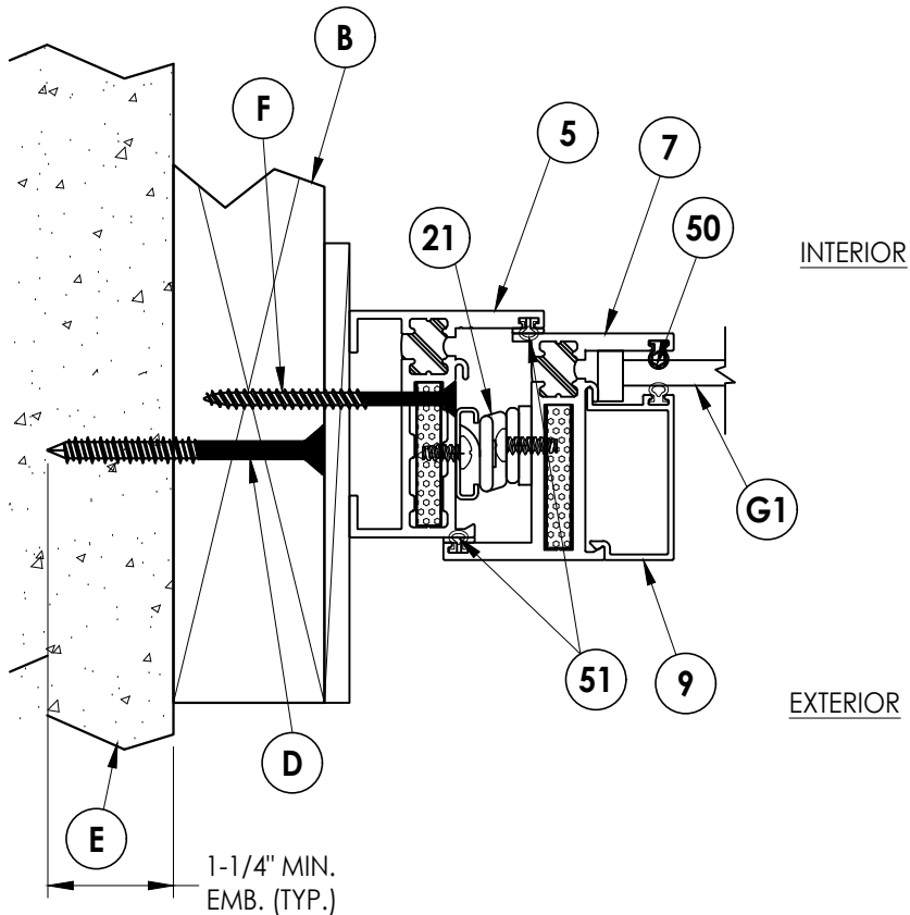
1 3 HORIZONTAL CROSS SECTION Shown w/ 2X Buck Construction
